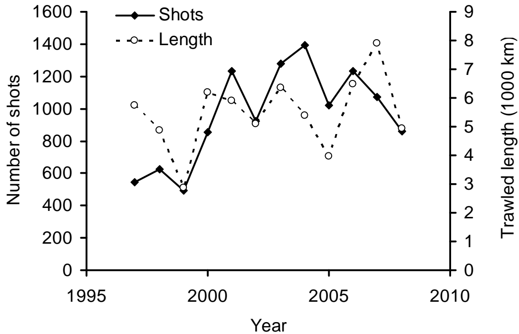
Figure 8-3. Fishing effort for the HIMI Demersal Trawl Sub-fishery from 1997 to 2008.
