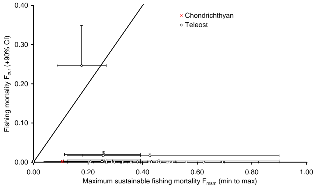
Figure 8-9. Comparison of estimated fishing mortality in the recent years (2004-2007) F_{cur} and the reference fishing mortality corresponding to the maximum sustainable mortality for fish species caught in the Macquarie Island Demersal Trawl Sub-fishery . The diagonal line is where F_{cur} = F_{msm} .
