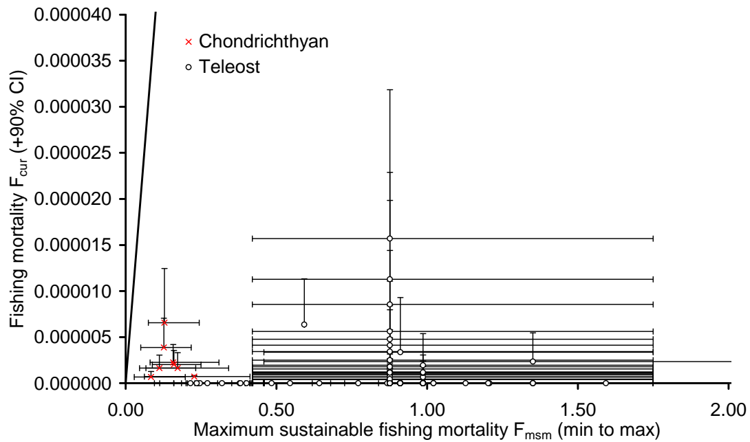
Figure 3-3. Comparison of estimated fishing mortality F_{cur} and the reference fishing mortality corresponding to the maximum sustainable mortality for fish species caught in the Skipjack Tuna Fishery . The diagonal line is where F_{cur} = F_{msm} .
