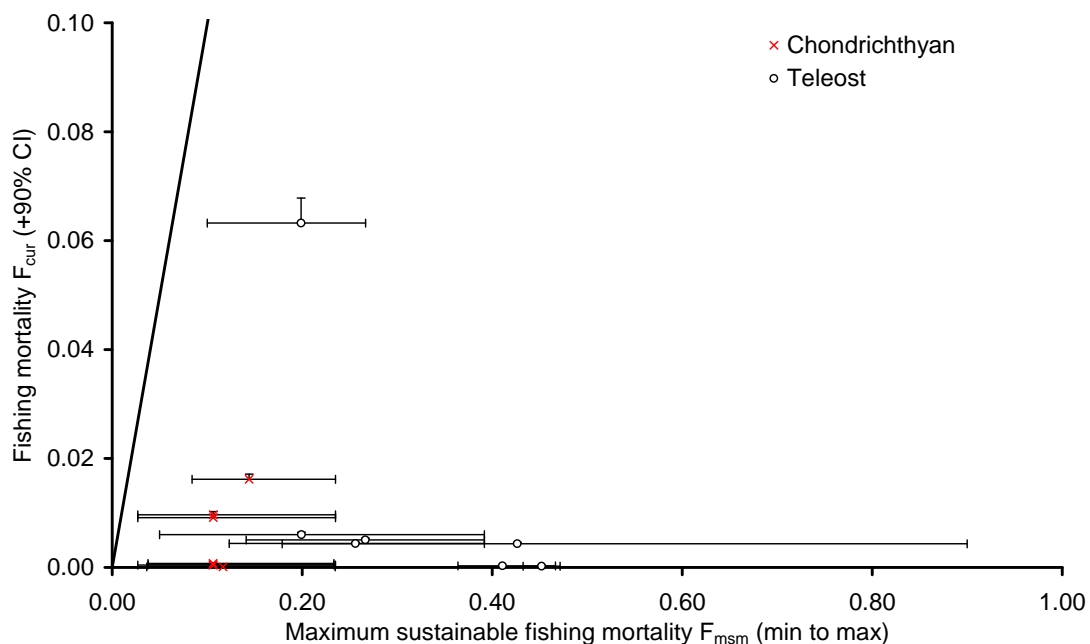
Figure 8-6. Comparison of estimated fishing mortality in the recent years (2004-2007) F_{cur} and the reference fishing mortality corresponding to the maximum sustainable mortality for fish species caught in the HIMI Demersal Demersal Longline Sub-fishery . The diagonal line is where F_{cur} = F_{msm} .
