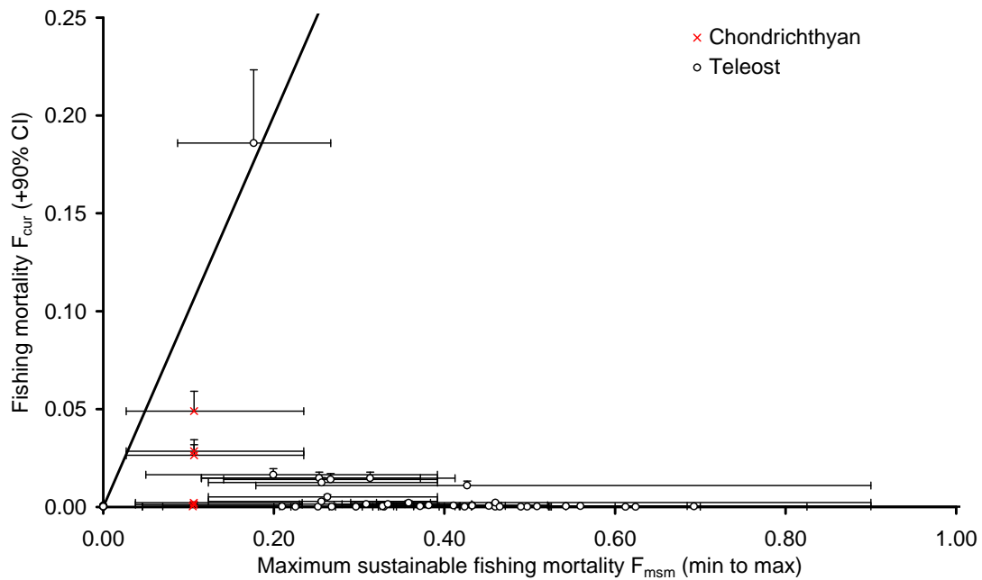
Figure 8-2. Comparison of estimated fishing mortality in the recent years (2004-2007) F_{cur} and the reference fishing mortality corresponding to the maximum sustainable mortality for fish species caught in the HIMI Demersal Trawl Sub-fishery . The diagonal line is where F_{cur} = F_{msm} . The species whose F_{cur} is above this diagonal line is Patagonian toothfish.
