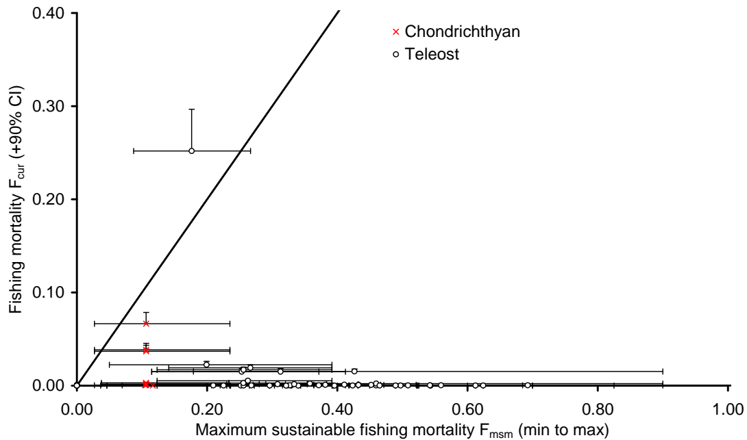
Figure 8-8. Comparison of estimated cumulative fishing mortality in recent years (2004-2007) F_{cur} and the reference fishing mortality corresponding to the maximum sustainable mortality for fish species caught in the three HIMI Sub-fisheries . The diagonal line is where F_{cur} = F_{msm} . The species whose F_{cur} is above this diagonal line is Patagonian toothfish.
