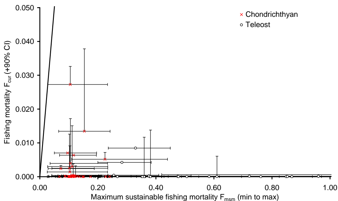
Figure 7-2. Comparison of estimated fishing mortality in the recent years (2004-2007) F_{cur} and the reference fishing mortality corresponding to the maximum sustainable mortality for fish species caught in the Western Tuna and Billfish Fishery . The diagonal line is where F_{cur} = F_{msm} .
