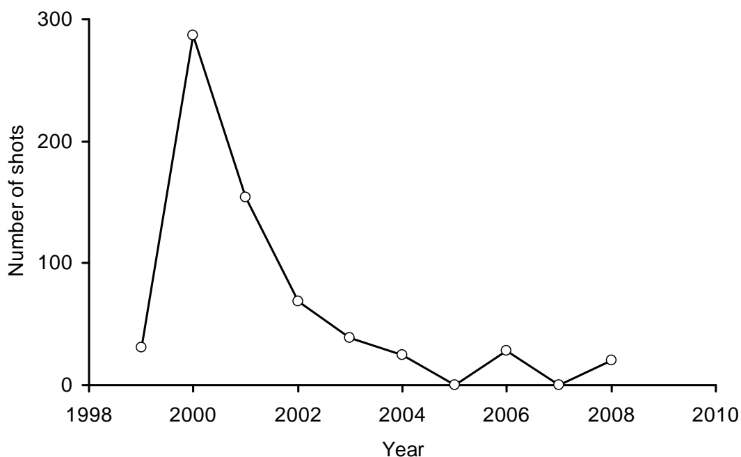
Figure 3-4. Fishing effort expressed as number of shots for the Skipjack Tuna Fishery from 1999 to 2008.
