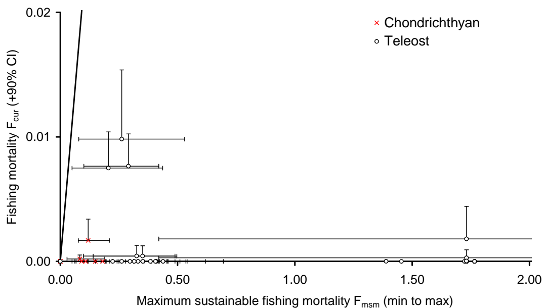
Figure 2-2. Comparison of estimated fishing mortality F_{cur} and the reference fishing mortality corresponding to the maximum sustainable mortality for fish species caught in the Northwest Slope Trawl Fishery . The diagonal line is where F_{cur} = F_{msm} .
