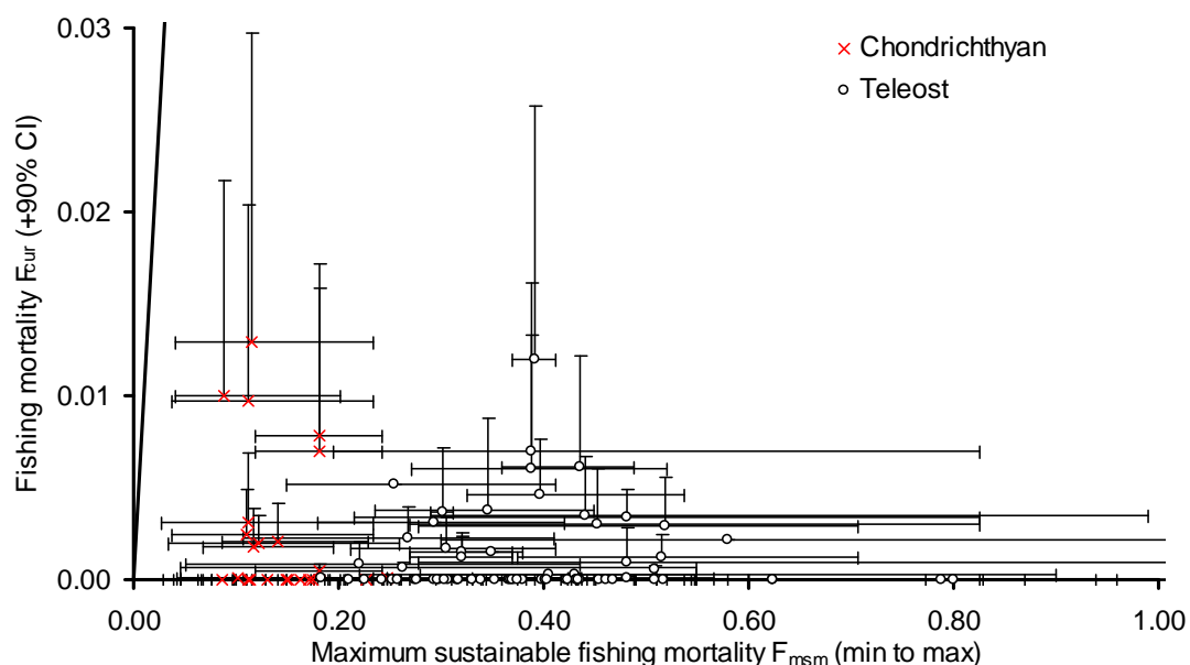
Figure 6-2. Comparison of estimated fishing mortality in the recent years (2004-2007) F_{cur} and the reference fishing mortality corresponding to the maximum sustainable mortality for fish species caught in the Western Deepwater Trawl Fishery . The diagonal line is where F_{cur} = F_{msm} .
