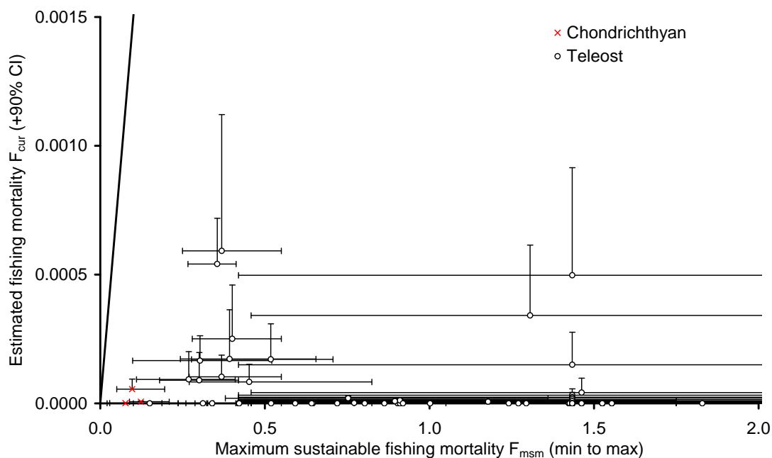
Figure 4-5. Comparison of estimated cumulative fishing mortality in the recent years (2004-2007) F_{cur} and the reference fishing mortality corresponding to the maximum sustainable mortality for fish species caught in the Small Pelagic Fishery . The diagonal line is where F_{cur} = F_{msm} .
