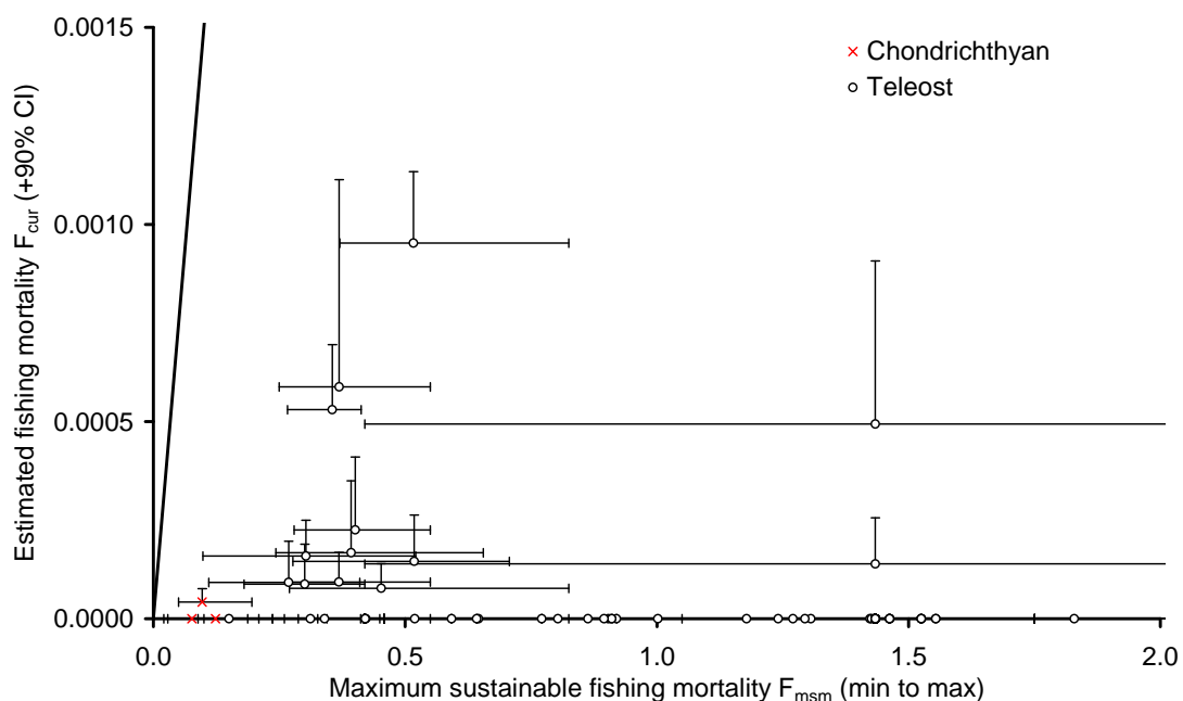
Figure 4-4. Comparison of estimated fishing mortality F_{cur} and the reference fishing mortality corresponding to the maximum sustainable mortality for fish species caught in the Mid-water Trawl Sub-fishery of the Small Pelagic Fishery . The diagonal line is where F_{cur} = F_{msm} .
