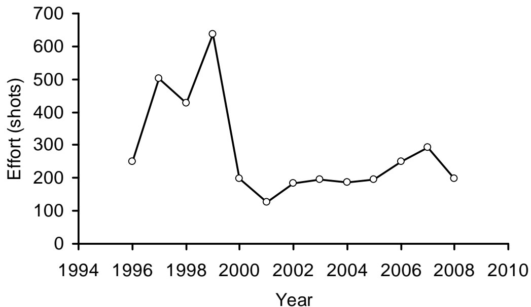
Figure 5-3. Fishing effort expressed as number of shots for the Southern Bluefin Tuna Fishery from 1996 to 2008.
