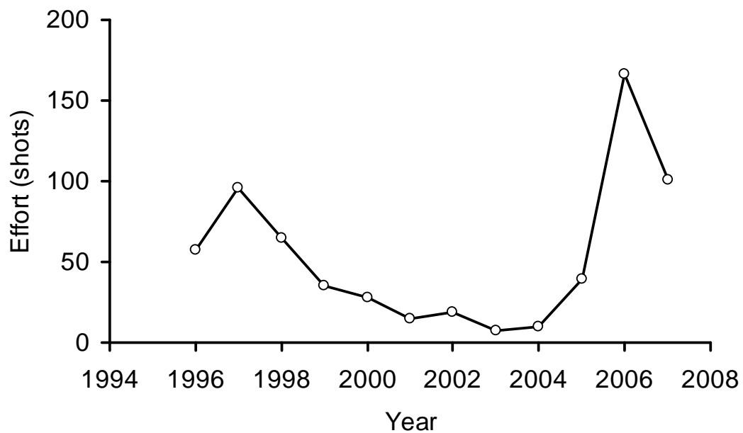
Figure 4-3. Fishing effort expressed as number of shots for the Purse Seine Sub-fishery of the Small Pelagic Fishery from 1996 to 2007.
