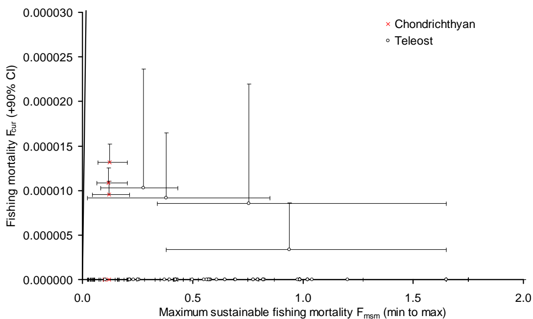
Figure 5-2. Comparison of estimated fishing mortality in the recent years (2004-2007) F_{cur} and the reference fishing mortality corresponding to the maximum sustainable mortality for fish species caught in the Southern Bluefin Tuna Fishery . The diagonal line is where F_{cur} = F_{msm} .
