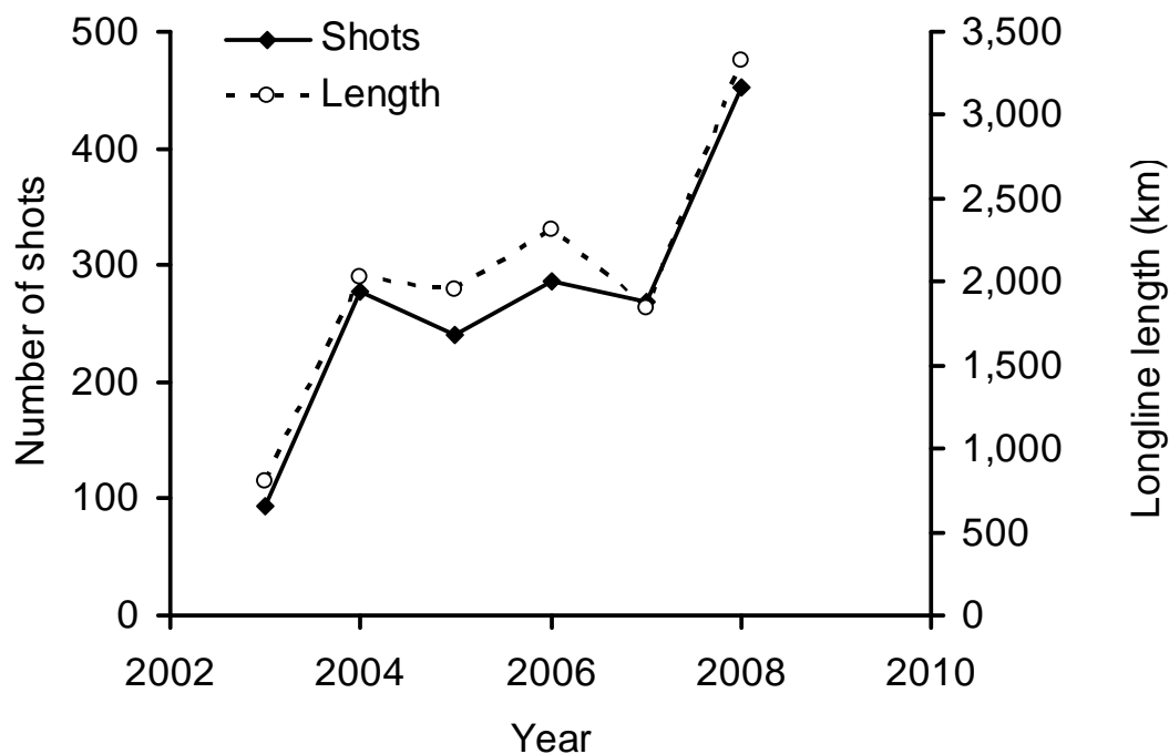
Figure 8-7. Fishing effort for the HIMI Demersal Longline Sub-fishery from 2003 to 2008.
