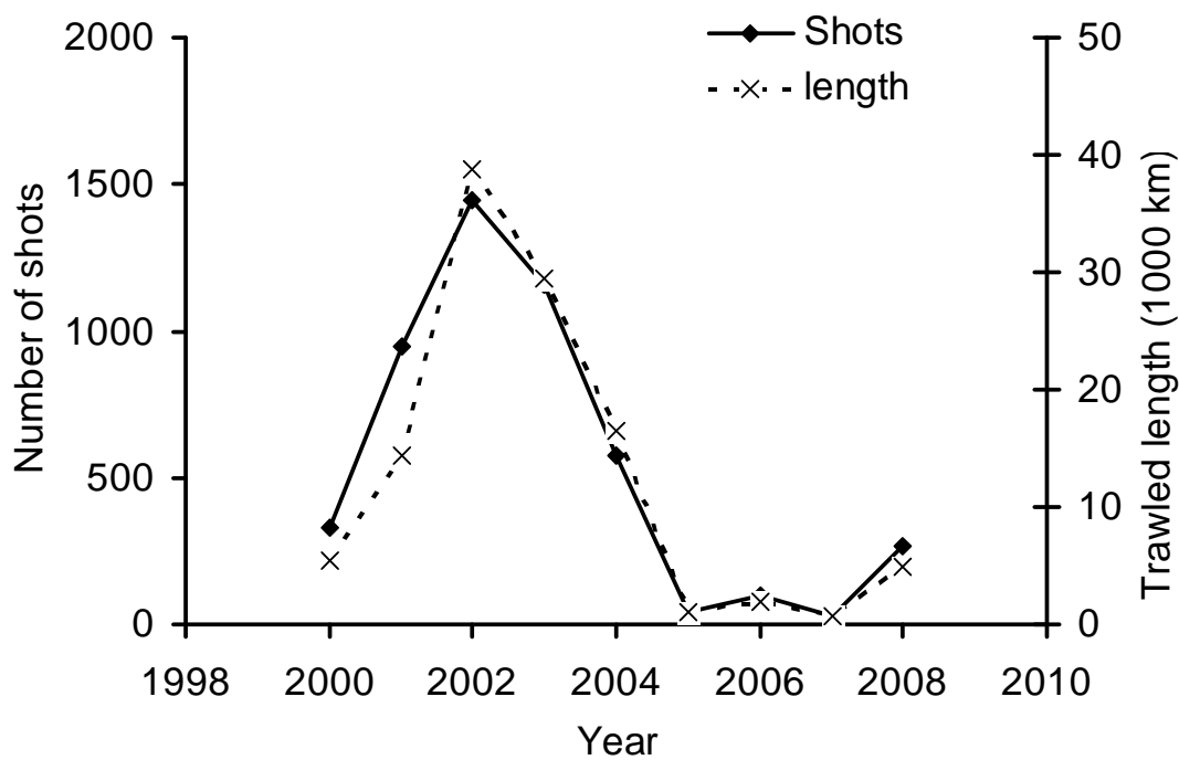
Figure 6-3. Fishing effort for the West Deepwater Trawl Fishery from 2000 to 2008.
