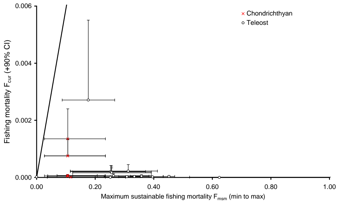
Figure 8-4. Comparison of estimated fishing mortality in the recent years (2004-2007) F_{cur} and the reference fishing mortality corresponding to the maximum sustainable mortality for fish species caught in the HIMI Mid-water Trawl Sub-fishery . The diagonal line is where F_{cur} = F_{msm} .
