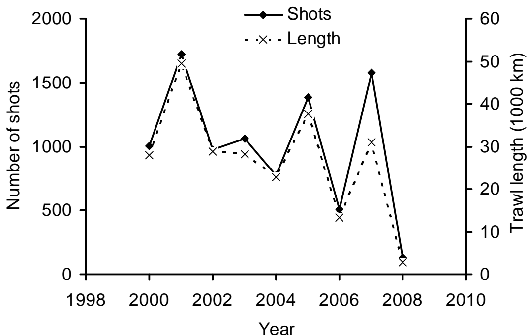
Figure 2-3. Fishing effort for the Northwest Slope Trawl Fishery from 2000 to 2008.
