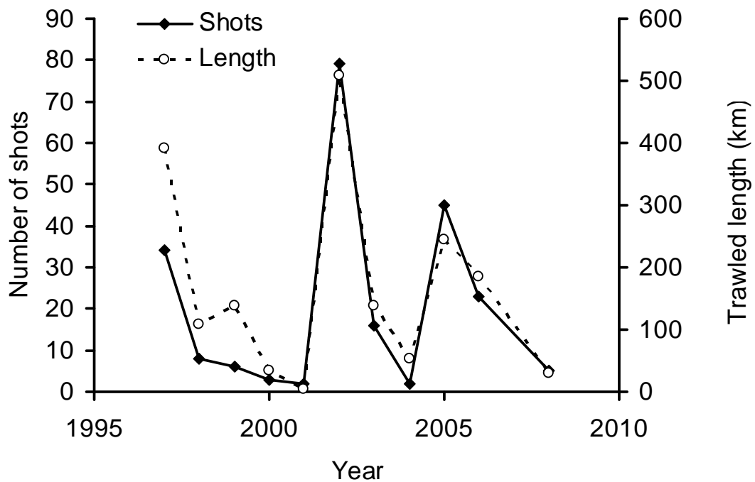
Figure 8-5. Fishing effort for the HIMI Mid-water Trawl Sub-fishery from 1997-2008.
