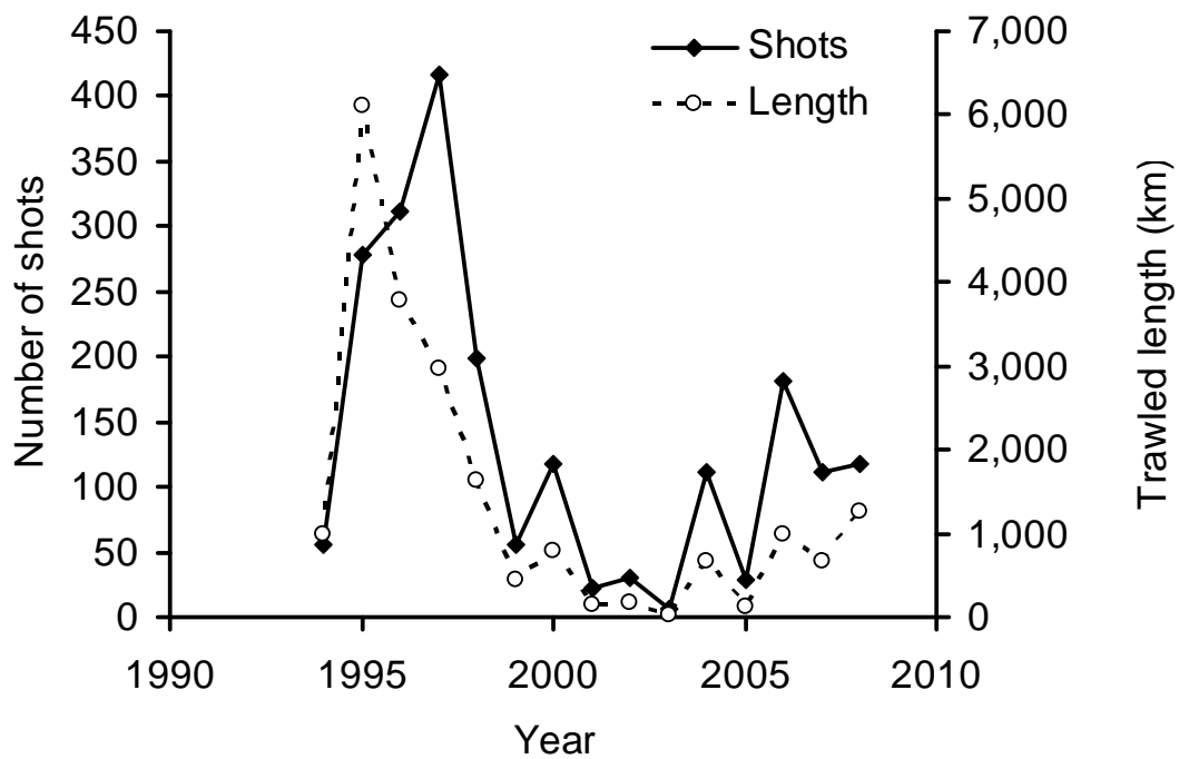
Figure 8-10. Fishing effort for the Macquarie Island Demersal Trawl Sub-fishery from 1994 to 2008.
