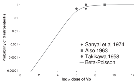
Figure I-9. Beta-Poisson dose-response curve for Vibrio parahaemolyticus .
