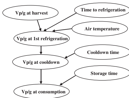
Figure I-6. Schematic depiction of the Post-harvest Module of the V. parahaemolyticus (Vp) risk assessment model.
