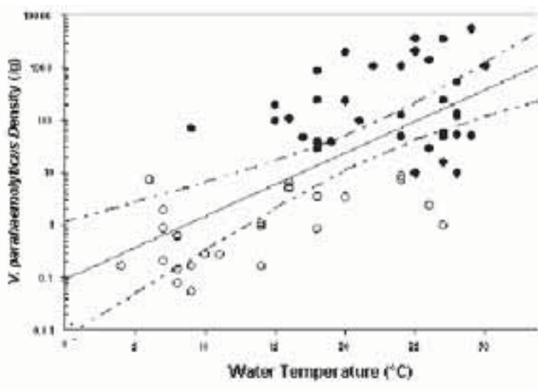
Figure I-3. Tobit regression fit of the Vibrio parahaemolyticus densities in oysters versus water temperature using the DePaola et al. (1990) data set. [Solid line is the best estimate of the median V. parahaemolyticus /g. Dashed lines show the 5th and 95th percentile confidence limits. Closed circles are V. parahaemolyticus detectable values from DePaola et al., (1990). Open circles are randomly imputed values for samples with densities less than the limit of detection (10 cfu/g).]
